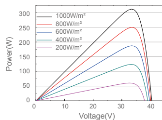
Power-Voltage Curve JAM60D00-310/BP
